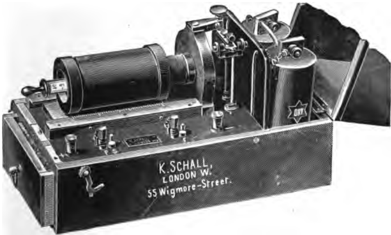
Dubois-Reymond's coil, with two dry cells.
